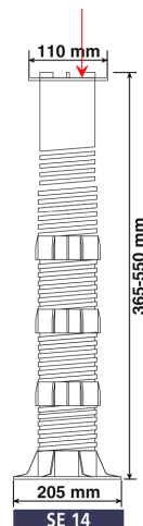
Figure 2 Typical "ETERNO SE14" specimen.
