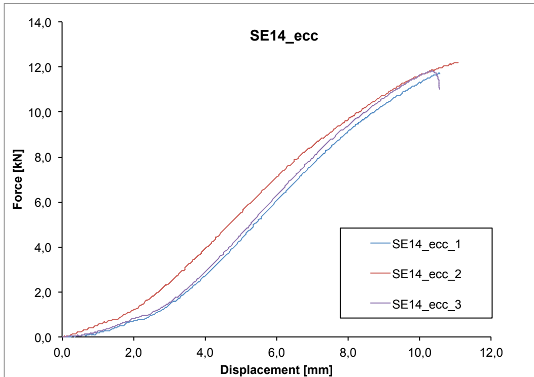
Figure 1 Diagram force versus displacement of testing machine's crossbar for "ETERNO SE14" specimen.
